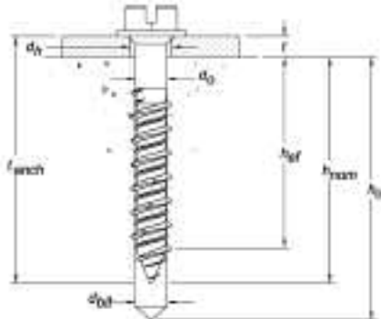
(Slotted hex head version pictured, flat head length measured from bottom of head to tip of anchor)
