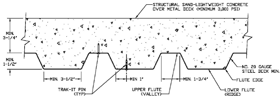
FIGURE 1—FASTENER INSTALLATION LOCATION ON COMPOSITE DECK
